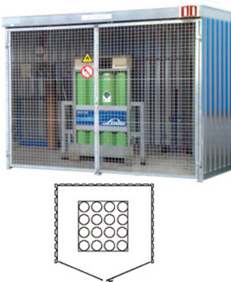
Size Hiltru Gas cylinder depot model GD3P- L
