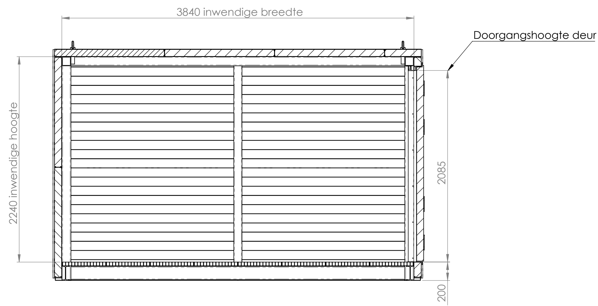
SECTION B-B SCALE 1 : 25
