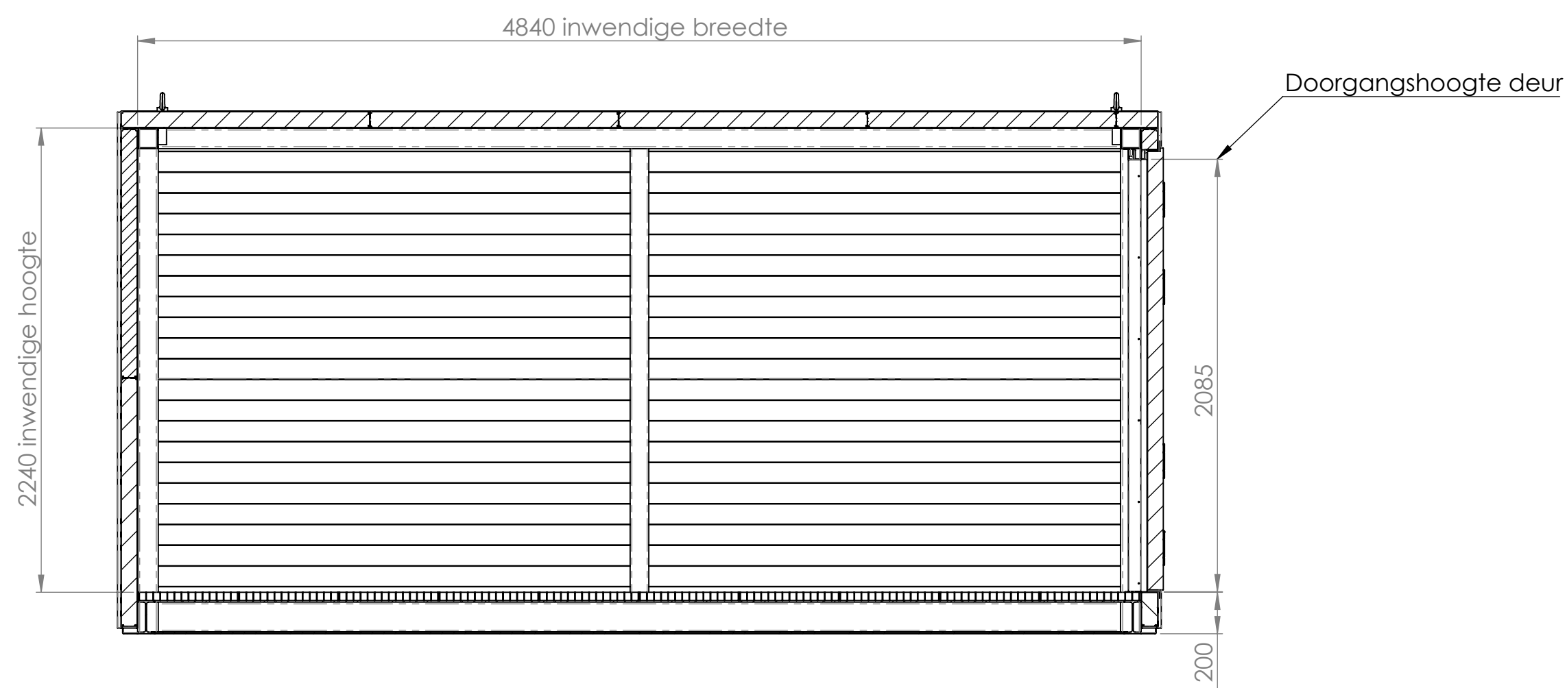
SECTION B-B SCALE 1 : 25
